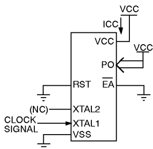
Figure 15. ICC Test Condition, Idle Mode. All Other Pins Are Disconnected.
