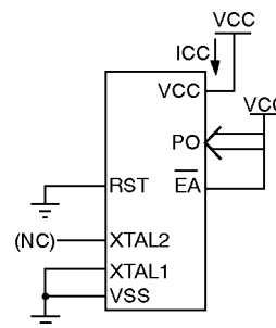
Figure 17. ICC Test Condition, Power Down Mode. All Other Pins Are Disconnected.
