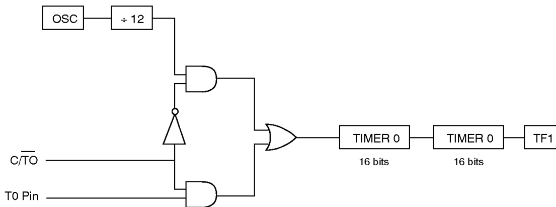
Figure 10. 32 Bit Timer/Counter.
